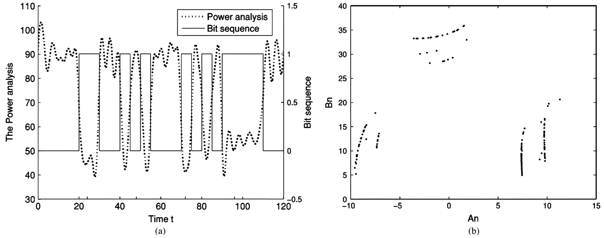
Fig. 1. For the transmitted signal generated by the classical parameter modulation: (a) bit sequence and the result of power analysis and (b) return map.
